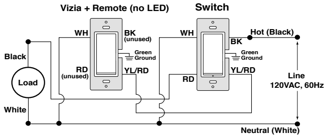
3-Way Wiring with VP0SR-10Z Coordinating Remote (no LED) Application:
