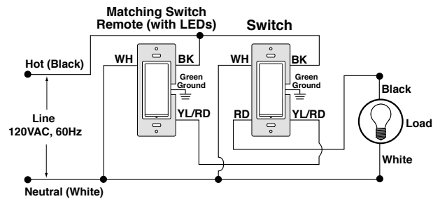
3-Way Wiring with VP0SR-1LZ Matching Remote (w/LEDs) Application:
